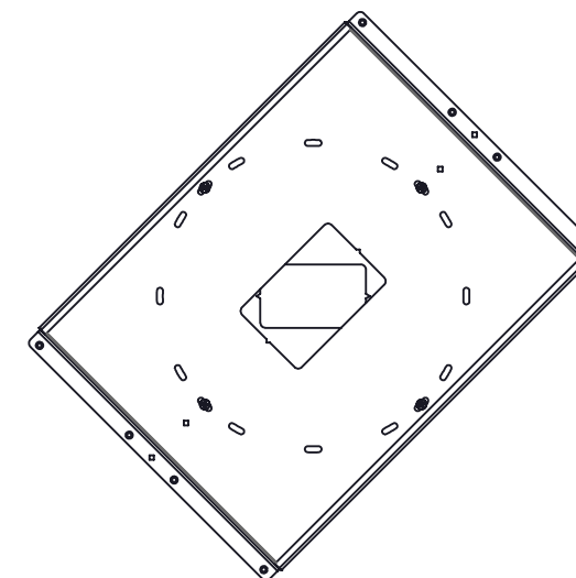
SHOWN AT 45°
