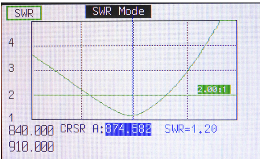
SWR
