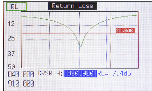
Return Loss
