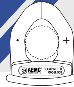
MODEL 505 Jaw Opening: 1.18" (30mm) Conductor Size: 500kcmil cable
