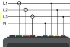
Three-phase 4 wires (L1, L2, L3, and N)
