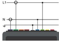
Single-phase 3 wires (L1, N, and earth)
