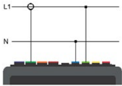
Single-phase 2 wires (L1 and N)
