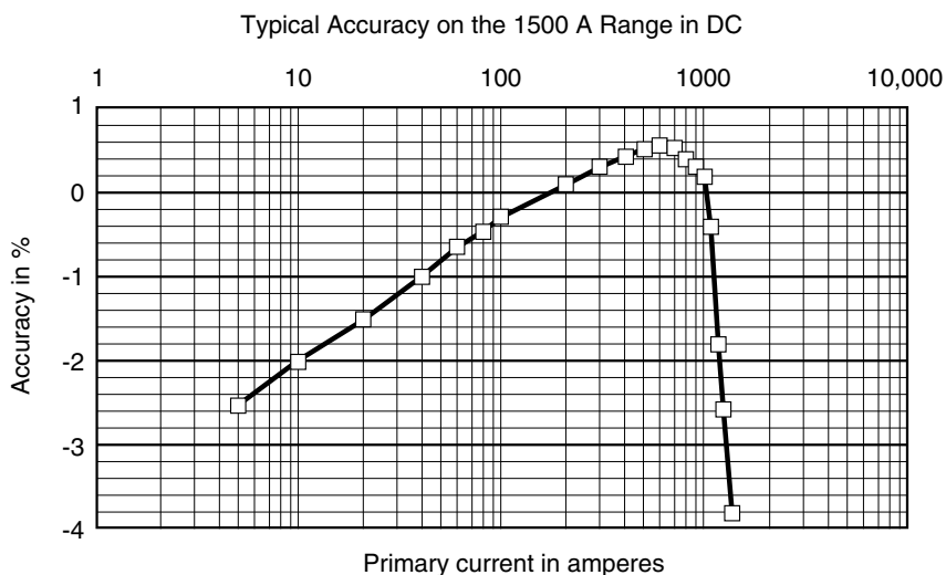
Typical Accuracy at 50 Hz: Range 1500 A (1 mV/A)
