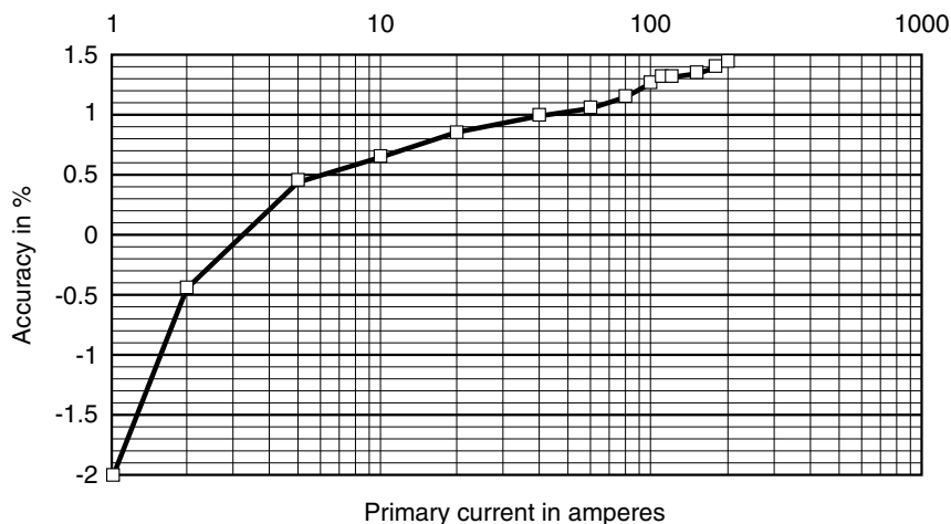
Typical Accuracy at 50 Hz: Range 150 A (10 mV/A)
