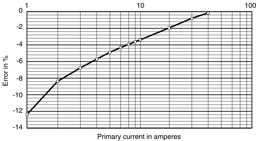
Typical Accuracy at 50 Hz: Range 60 A (10 mV/A)
