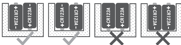
FIGURE 2-2. BATTERY POLARITY
