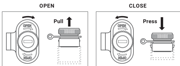
FIGURE 2-1. BATTERY COMPARTMENT
