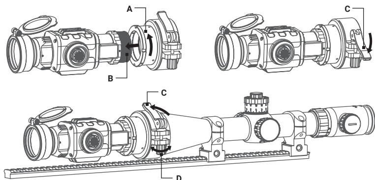
FIGURE 2-4. CLIP-ON INSTALLATION
