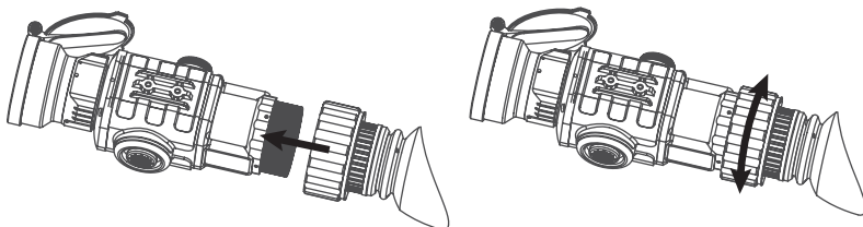
FIGURE 2-7. TRANSFORM TO MONOCULAR
