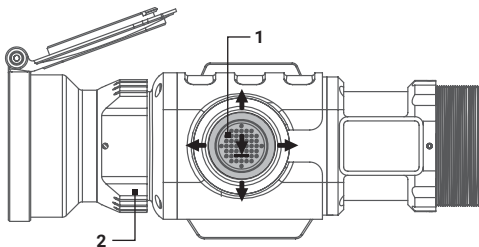
FIGURE 2-8. CONTROLS
