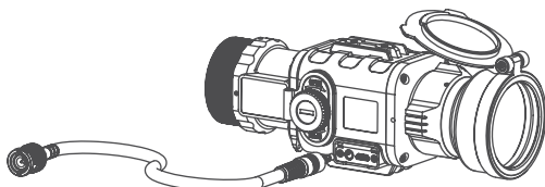
FIGURE 2-5. CABLE CONNECTION
