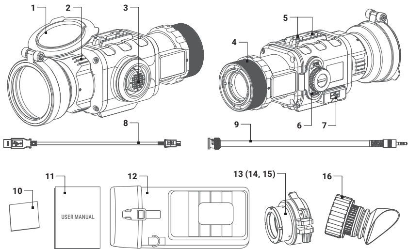
FIGURE 1-1. ANACONDA-MICRO TC50 MAIN PARTS AND COMPONENTS
