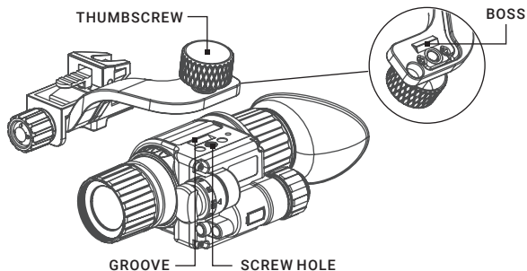
FIGURE 2-2. J-TYPE ADAPTER INSTALLATION
