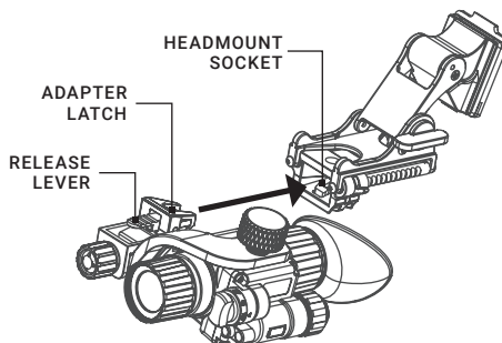
FIGURE 2-4. MOUNTING THE WOLF-14 TO A HELMET MOUNT
