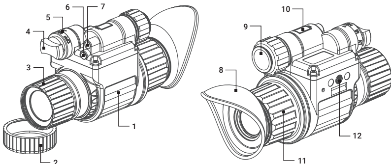
FIGURE 1-1. WOLF-14 MAIN PARTS
