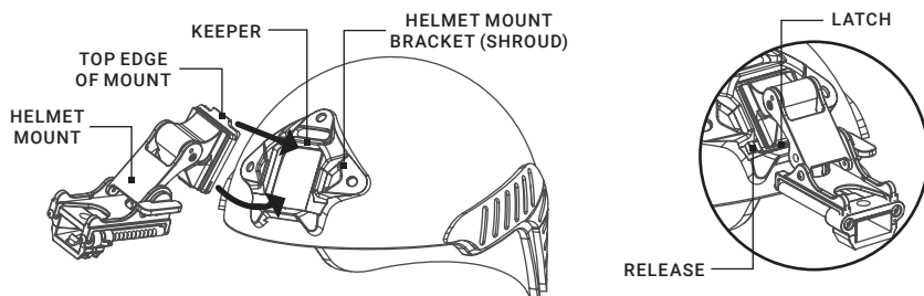
FIGURE 2-3. MOUNTING THE HELMET MOUNT TO A HELMET
