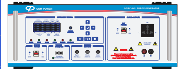
SGIEC-645 Surge Generator 1.2/50 µs, 8/20 µs Combination Wave 10/700 µs, 5/320 µs Combination Wave
