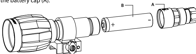
FIGURE 3-3. XLR-IR850 ILLUMINATOR. BATTERY INSTALLATION
