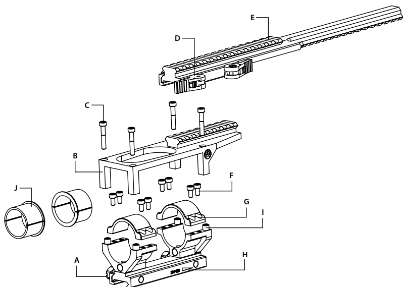
FIGURE 3-7. OPTIONAL FSRS SYSTEM. COMPONENT PARTS
