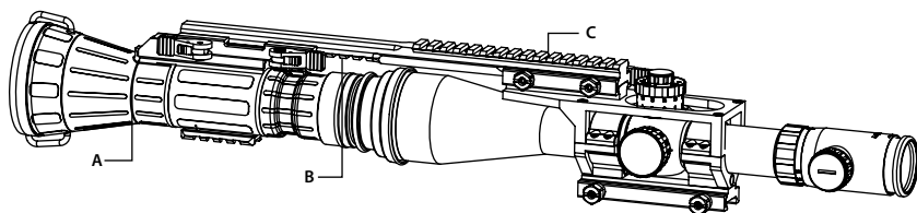
FIGURE 3-9. CO-LR AND DAY SCOPE MOUNTED ON FSRs SYSTEM
