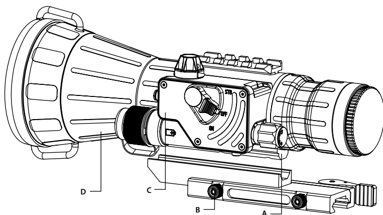
FIGURE 2-1. CO-LR NIGHT VISION CLIP-ON SYSTEM
