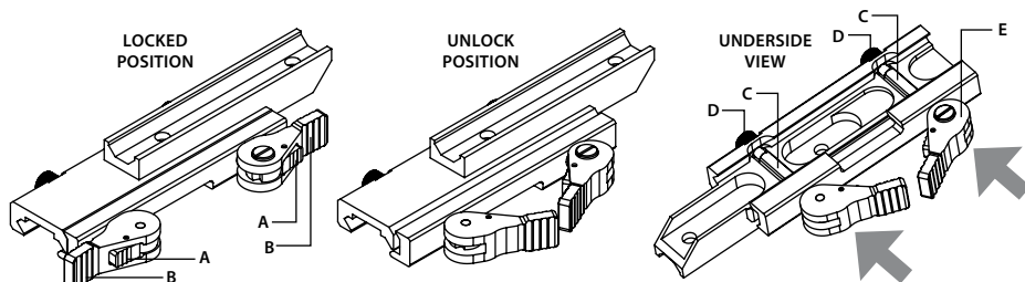
FIGURE 3-6. CO-LR MOUNT
