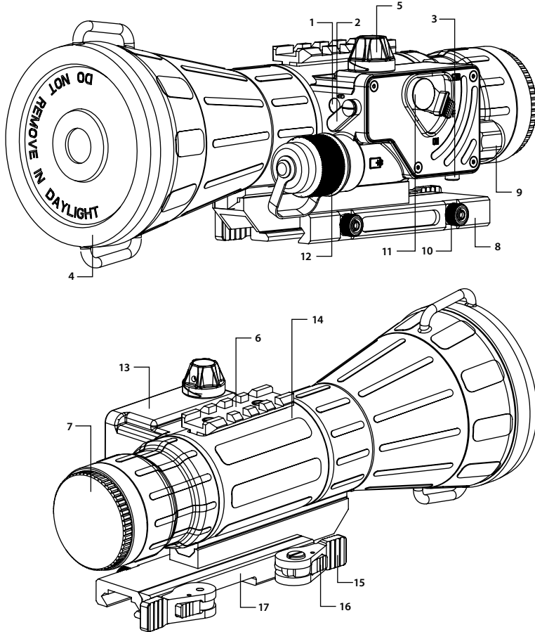
FIGURE 2-2. CO-LR NIGHT VISION CLIP-ON SYSTEM
