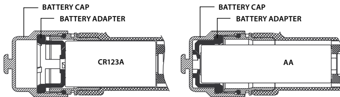
FIGURE 3-2. BATTERY ADAPTER POSITIONS IN THE BATTERY CAP
