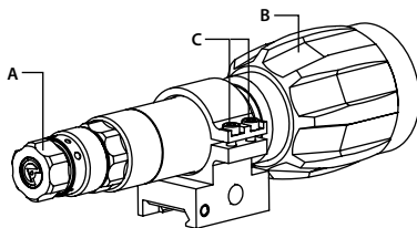
FIGURE 3-14. IR ILLUMINATOR ADJUSTMENT
