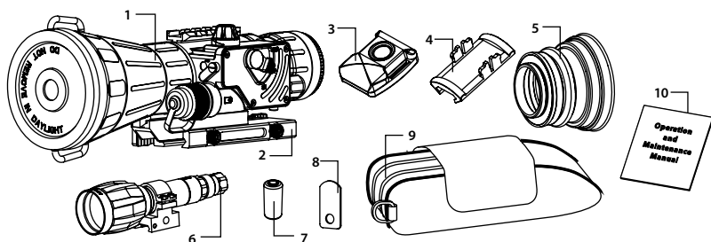
FIGURE 2-3. CO-LR STANDARD COMPONENTS
