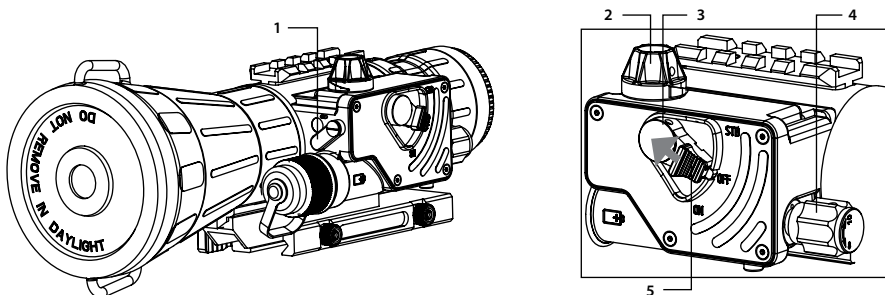
FIGURE 3-12. CO-LR CONTROLS
