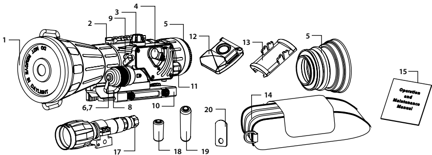
FIGURE B-1. CO-LR SPARE PARTS
