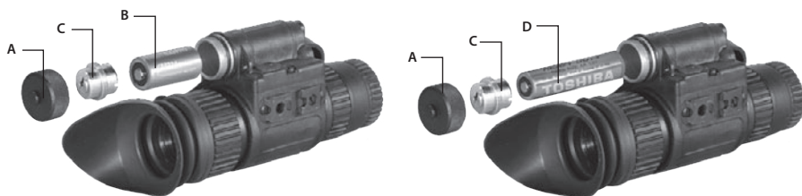
FIGURE 3-1. BATTERY INSTALLATION
