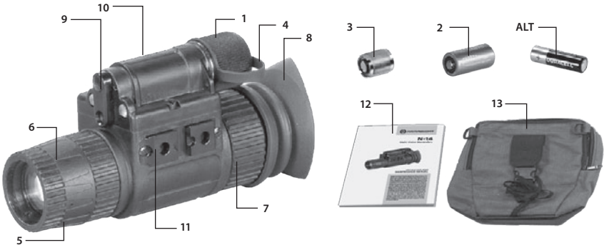
FIGURE A-1. N-14 SPARE PARTS
