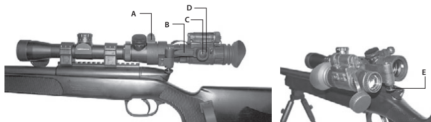
FIGURE 3-6. MOUNTING THE N-14 TO A SCOPE
