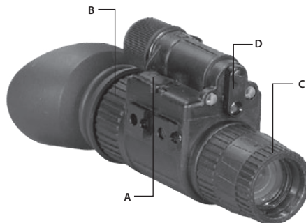
FIGURE 3-13. N-14 CONTROLS
