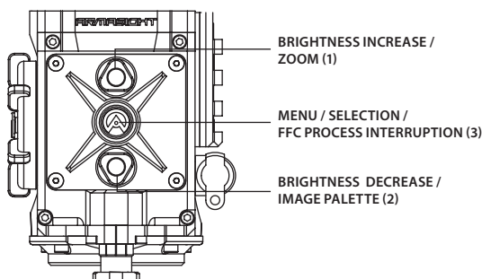
FIGURE 3-17. SETTING BUTTONS
