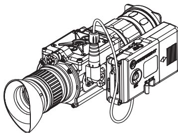
FIGURE 3-4. ARMASIGHT DIGITAL RECORDER DT INSTALLATION
