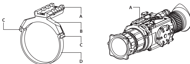
FIGURE 3-2. PLATFORM RING
