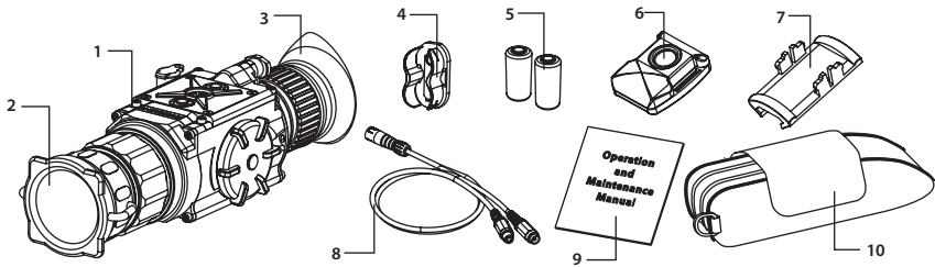
FIGURE 2-3. STANDARD COMPONENTS
