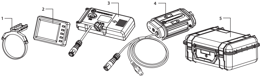
FIGURE 2-4. OPTIONAL EQUIPMENT
