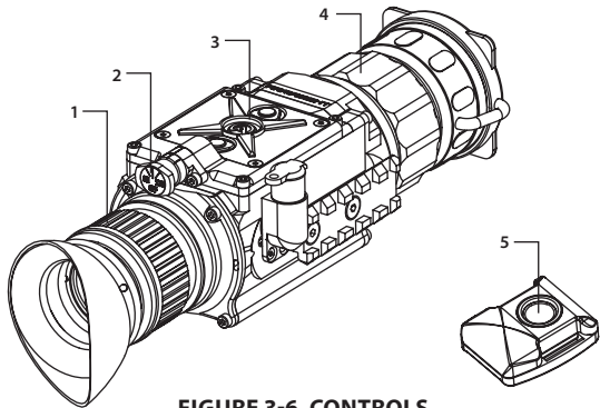
FIGURE 3-6. CONTROLS
