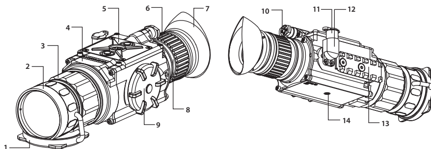
FIGURE 2-2. PROMETHEUS THERMAL IMAGING MONOCULAR. SYSTEM DESCRIPTION
