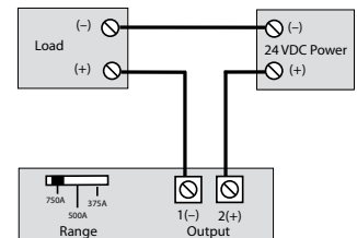
Alternate Connection
