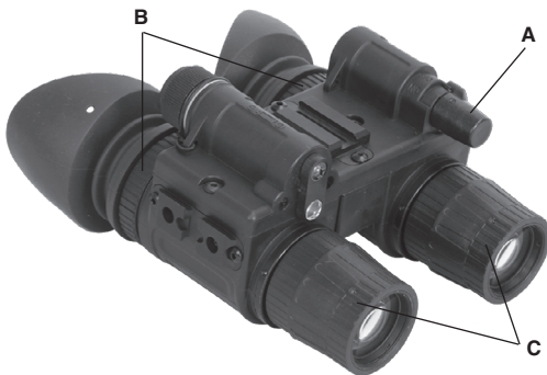
FIGURE 4-3. MECHANICAL FUNCTIONS
