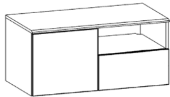
Left Hand Wall Mounted Unit 42.375"W x 22"D x 19.375"H
