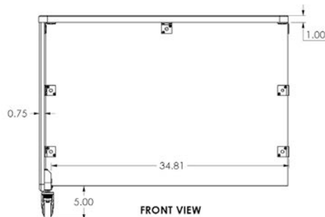
Left hand application shown. Parts can be used for right hand application
