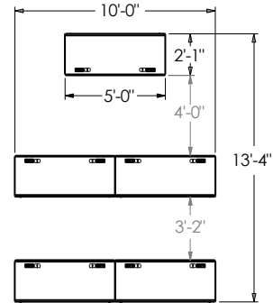
MFT6024-2P 60"W x 24.75"D x 30.75"H
