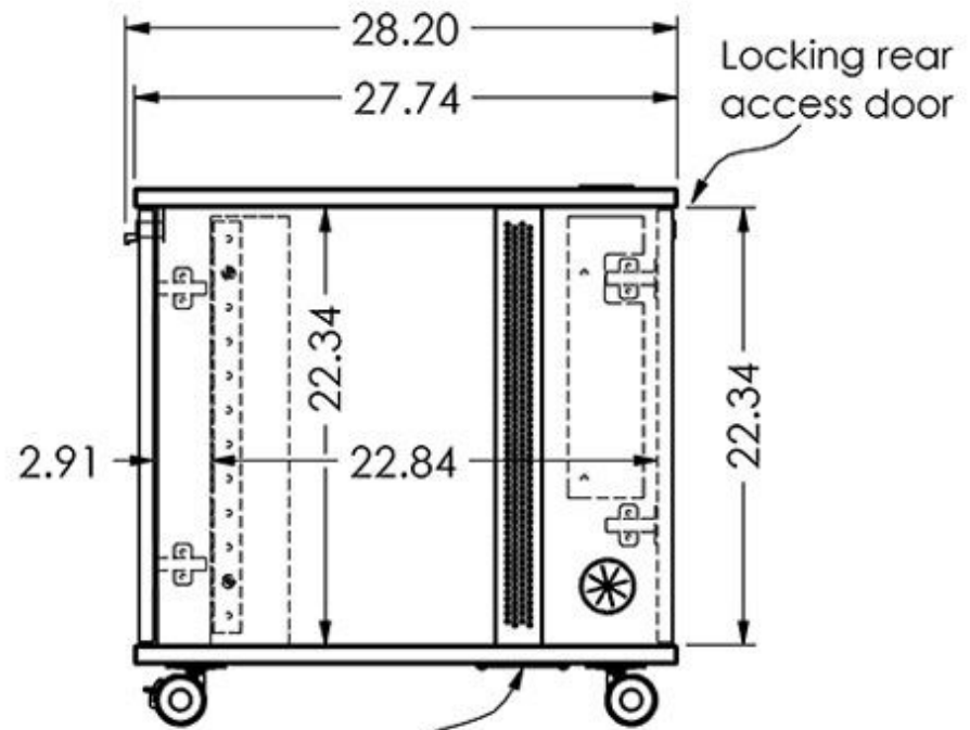
Bottom cutouts for fan and cable access
