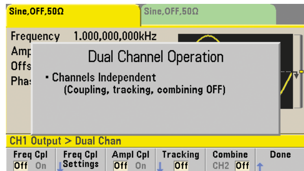
Figure 1. You can access the 33522A waveform generator's dual-channel settings via the softkey menu. The Dual Channel Operation menu allows you to adjust settings for frequency coupling, amplitude coupling, tracking and combining waveforms.
