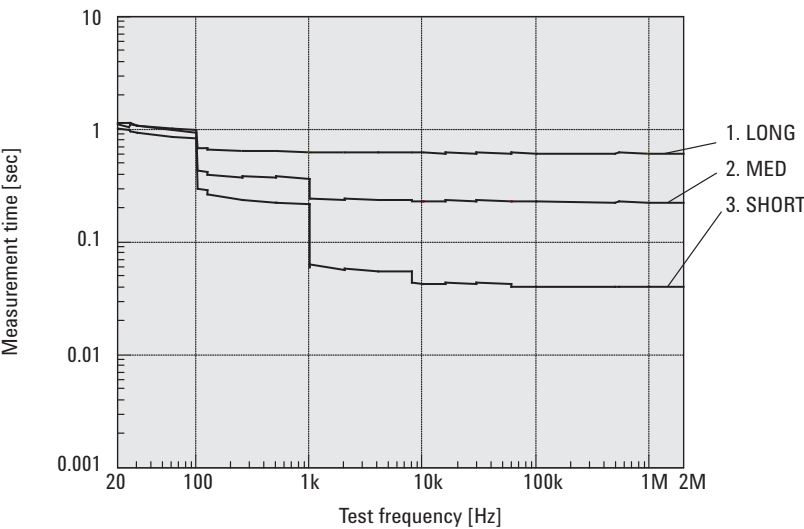
Figure 10. Measurement time (DC bias: OFF, E4980A-005)
