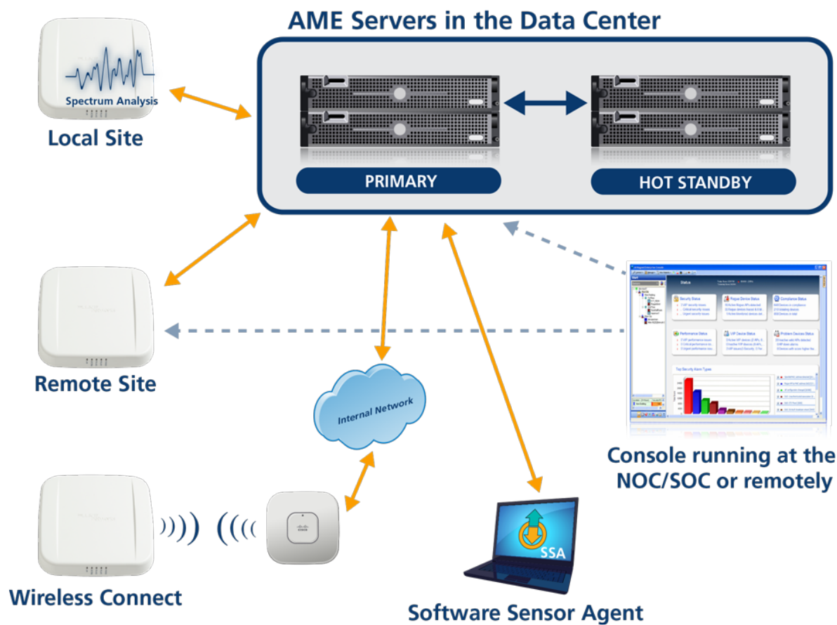
AirMagnet Enterprise System
