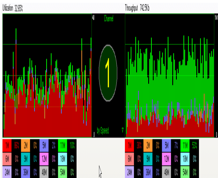
AirMagnet WiFi Analyzer Console screen shot on Bandwidth Utilization, Throughput, and Transmit Speed Relationship
