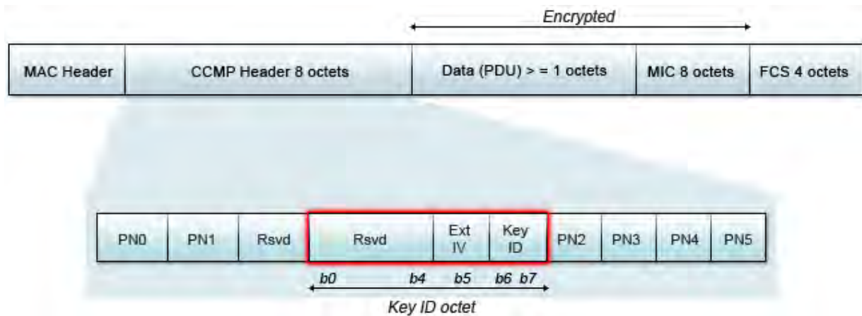
CCMP MPDU
