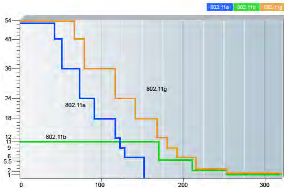
802.11 a/b/g Speed and Range Correlation
