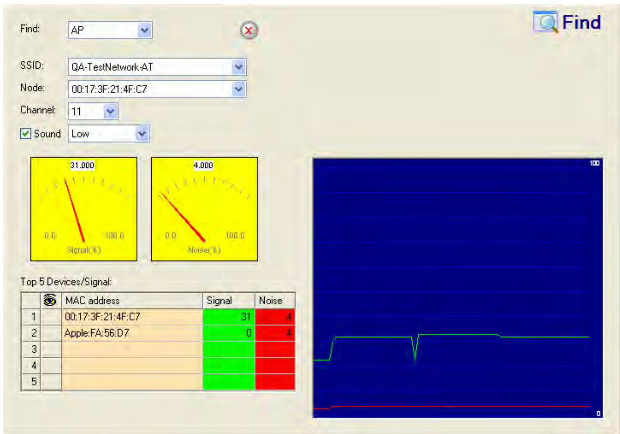
AirMagnet WiFi Analyzer's Find Tool used for locating an intruding device
