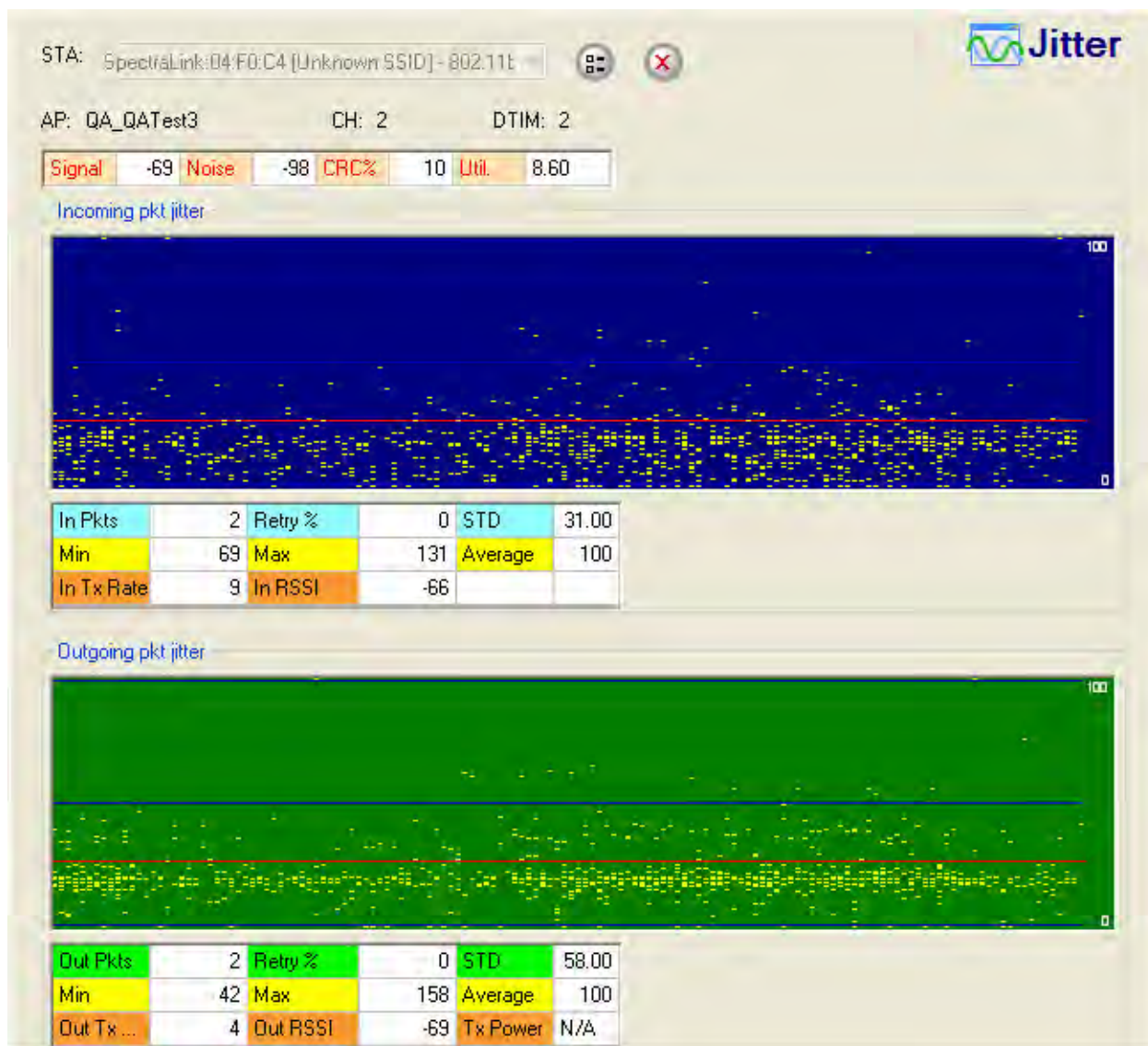
AirMagnet Jitter tool to measure jitter
