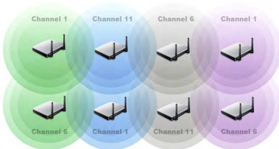
Site Survey Allocate Non-overlapping Channels to Physically Adjacent APs
