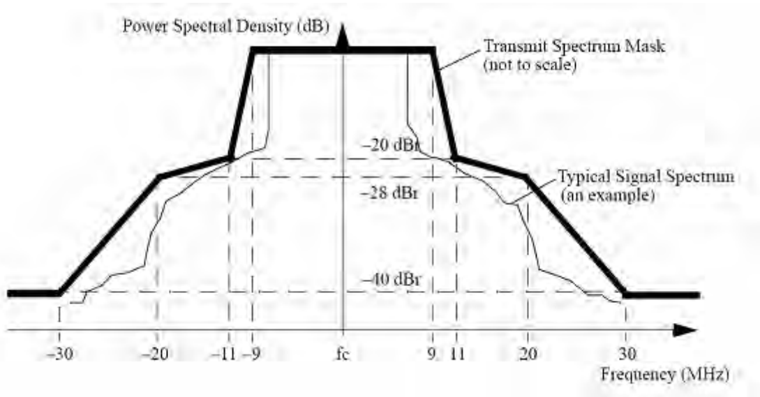
Transmit Spectrum Mask for 802.11a/g (20 MHz)
