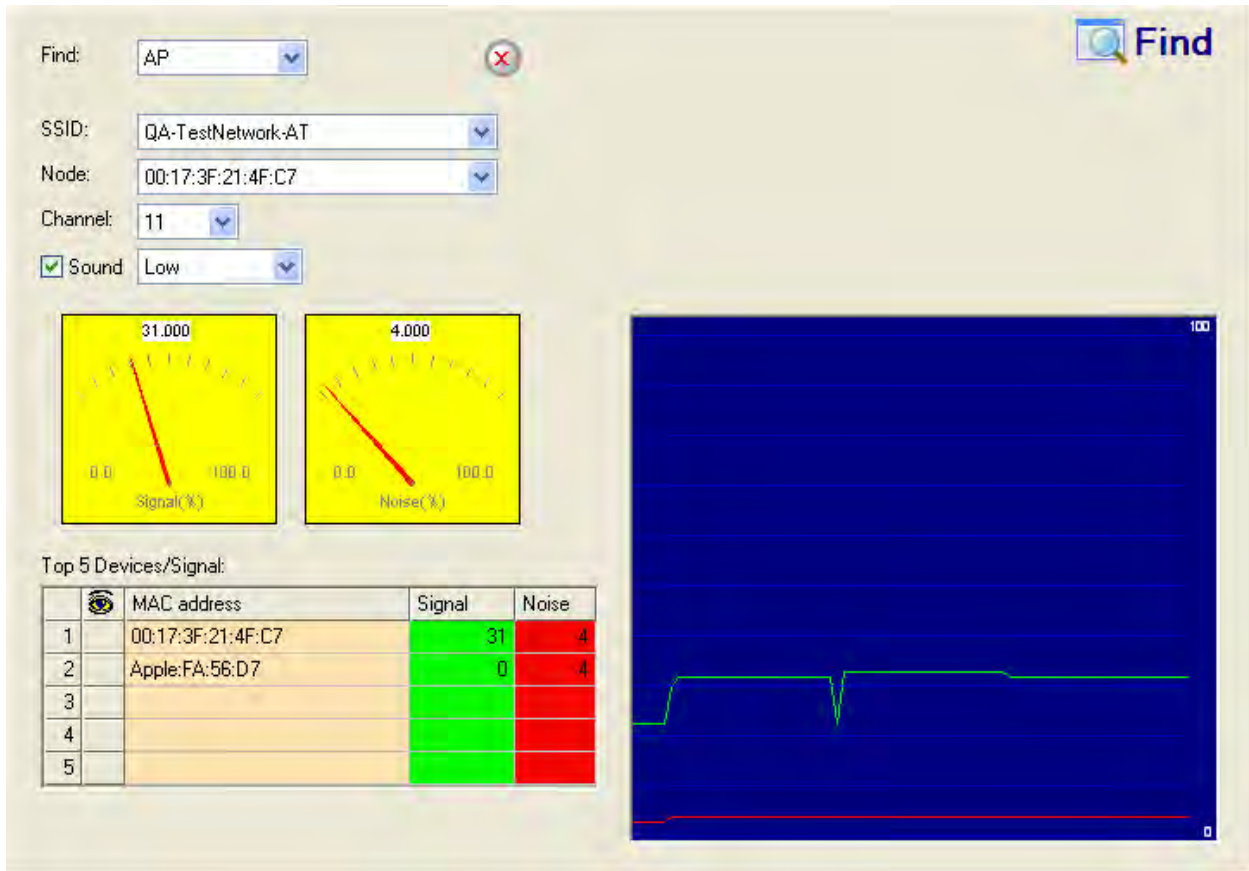
AirMagnet WiFi Analyzer's Find tool locates a device by tracking its signal and noise level
