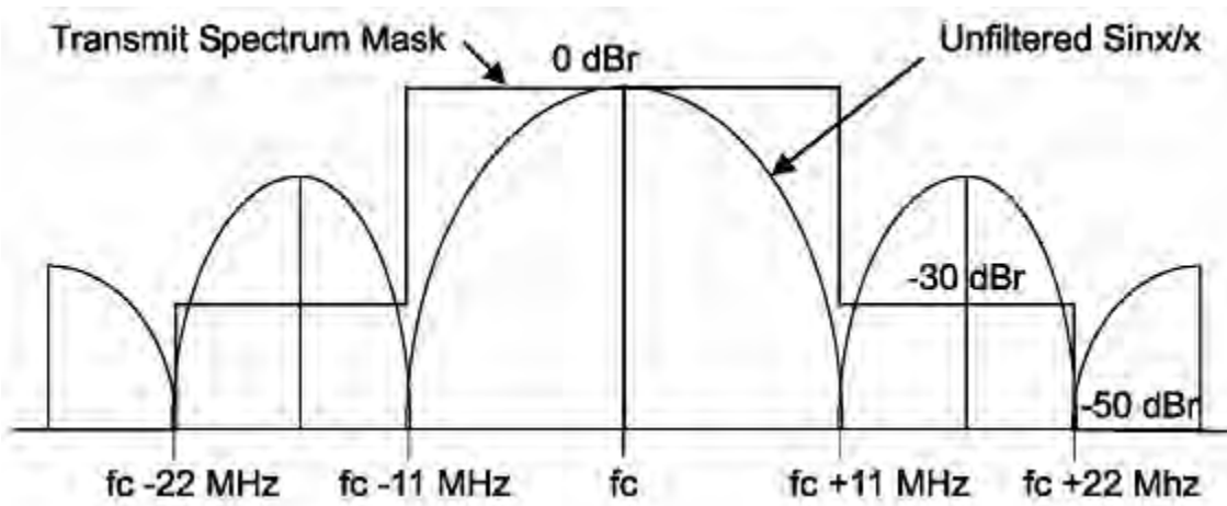
Transmit Spectrum Mask for 802.11b
