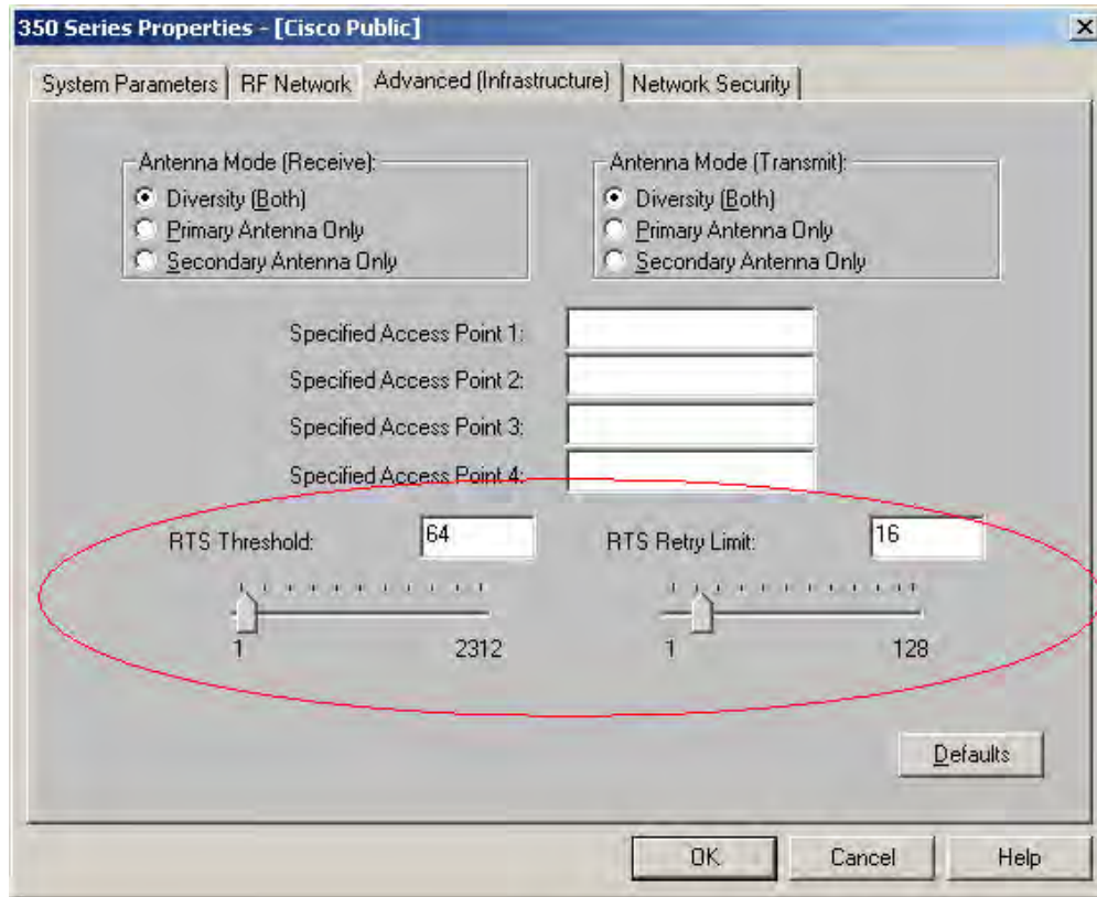
Sample RTS/CTS Configuration for a Cisco Aironet Client Adapter to Resolve the Hidden Node Problem
