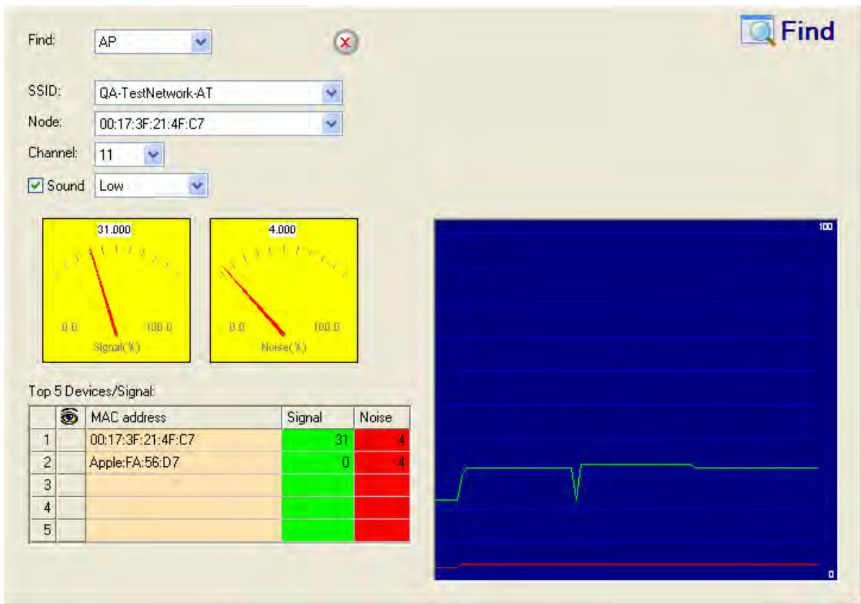
AirMagnet WiFi Analyzer's FIND tool locates devices by tracking down their signal level
