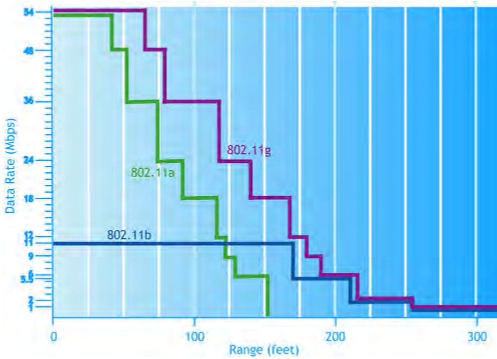
802.11 a/b/g Speed and Range Correlation
