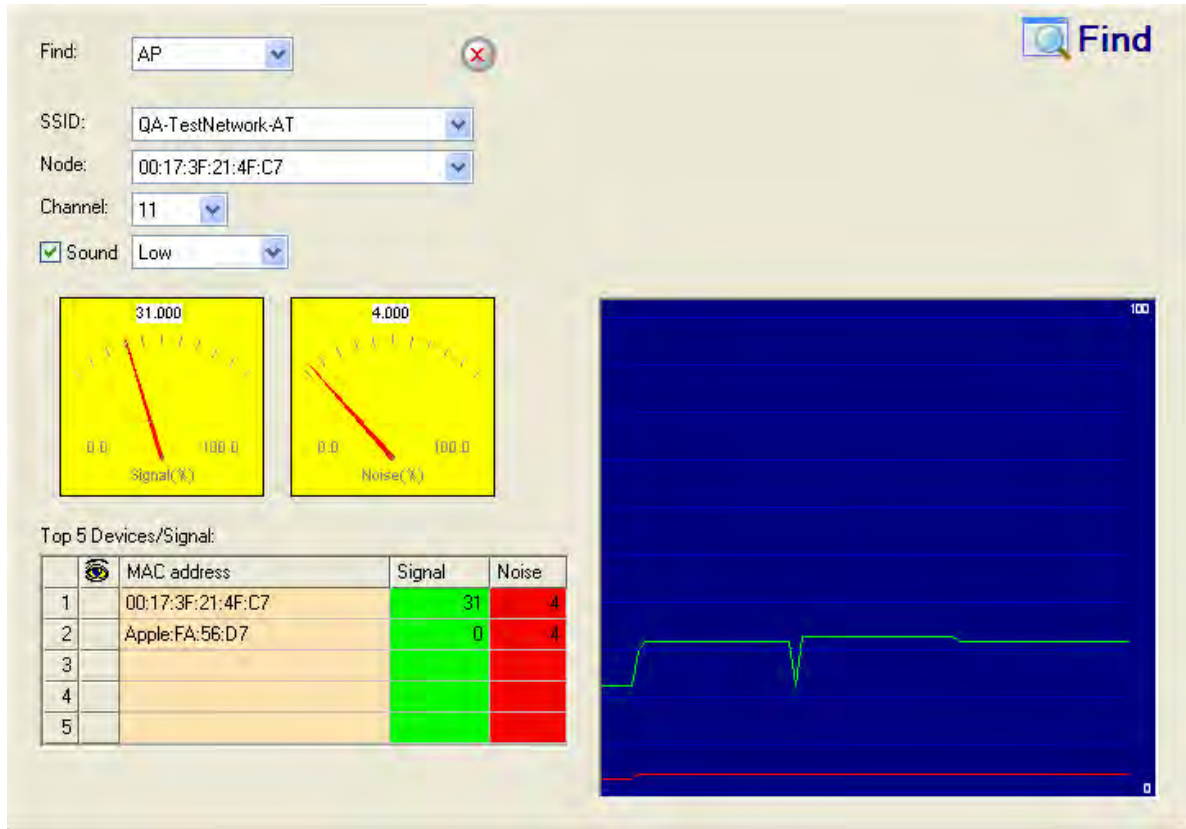
AirMagnet WiFi Analyzer's Find tool locating the source of an RTS flood attack
