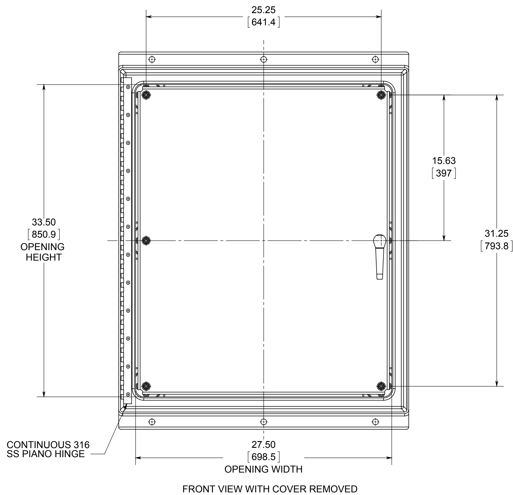
FRONT VIEW WITH COVER REMOVED
