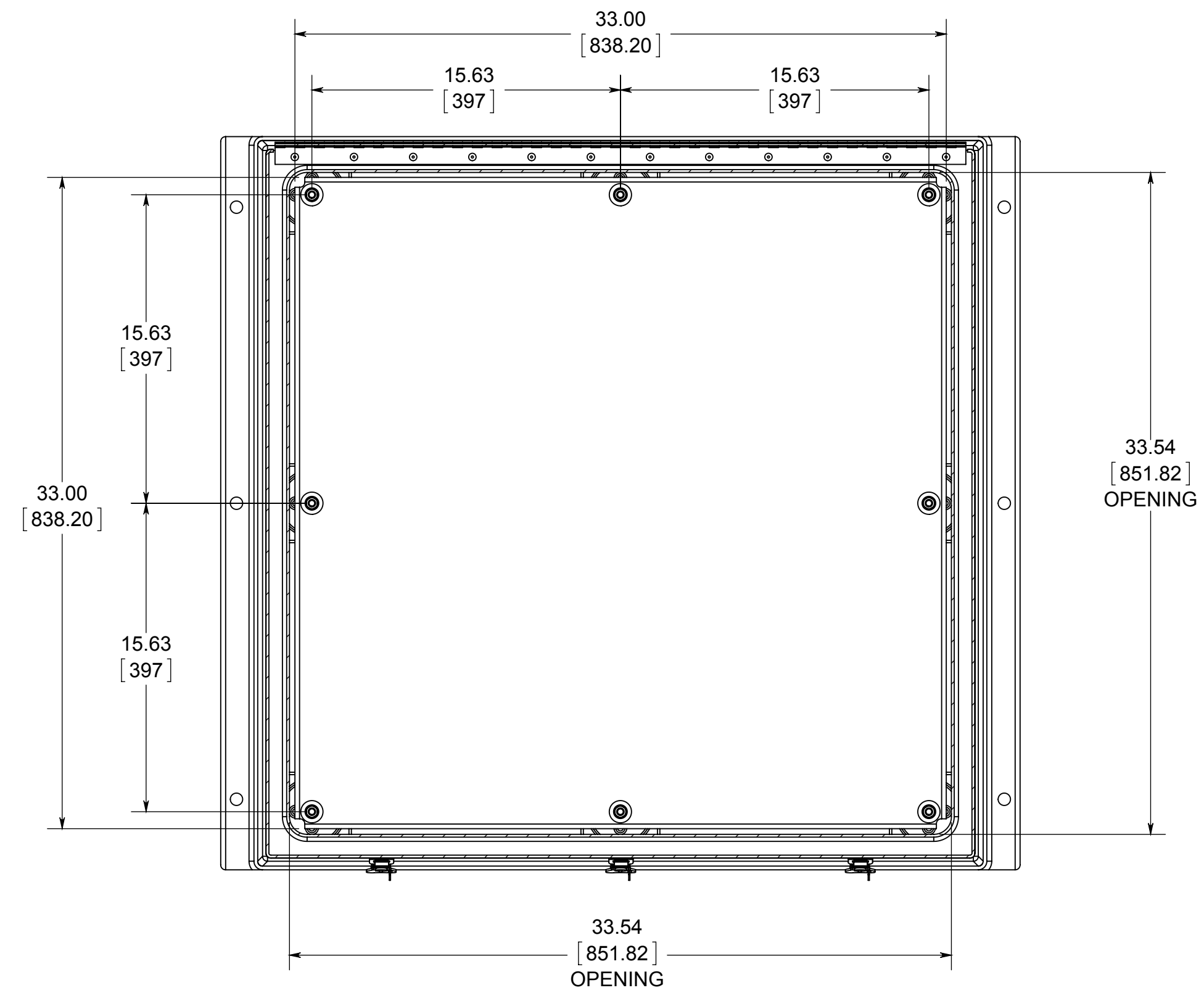
VIEW WITH LID & GASKET REMOVED
