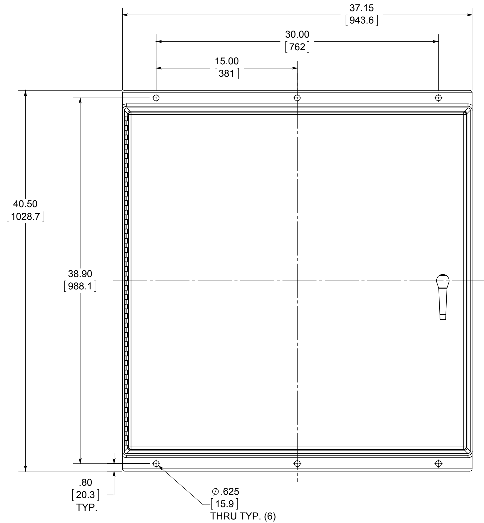
FRONT VIEW WITH COVER
