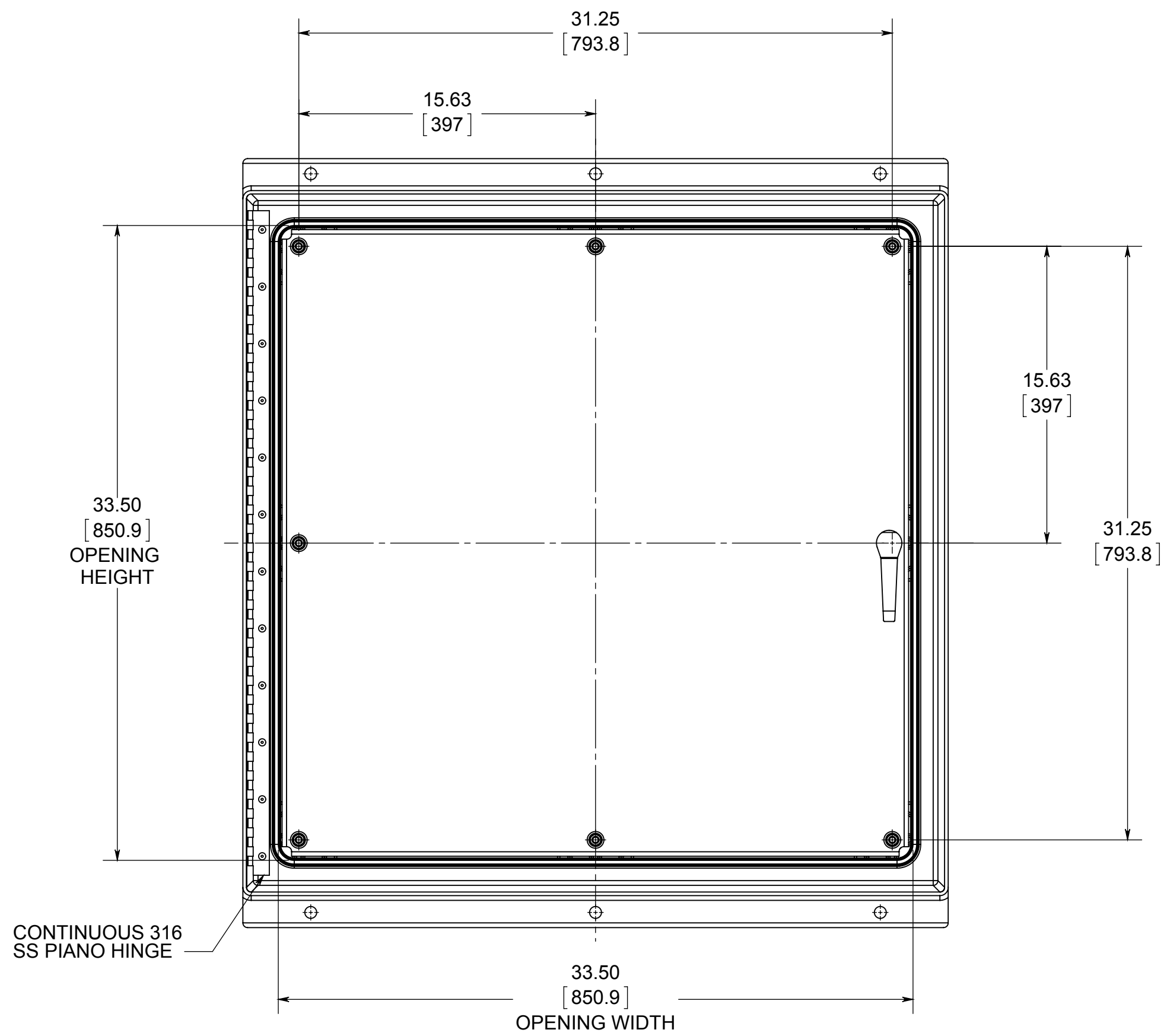
FRONT VIEW WITH COVER REMOVED
