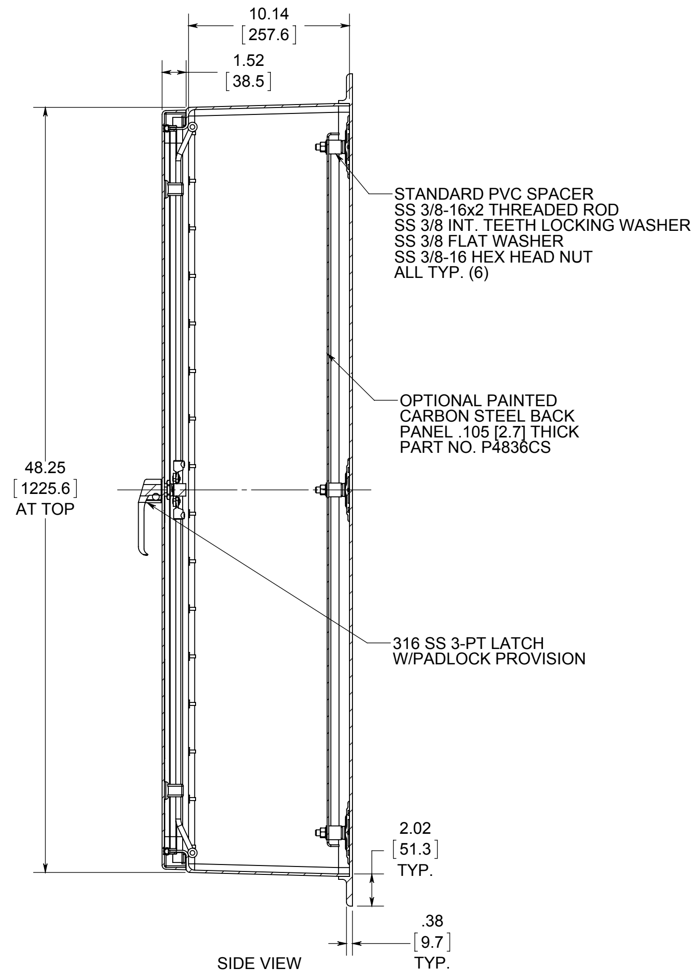
SIDE VIEW
