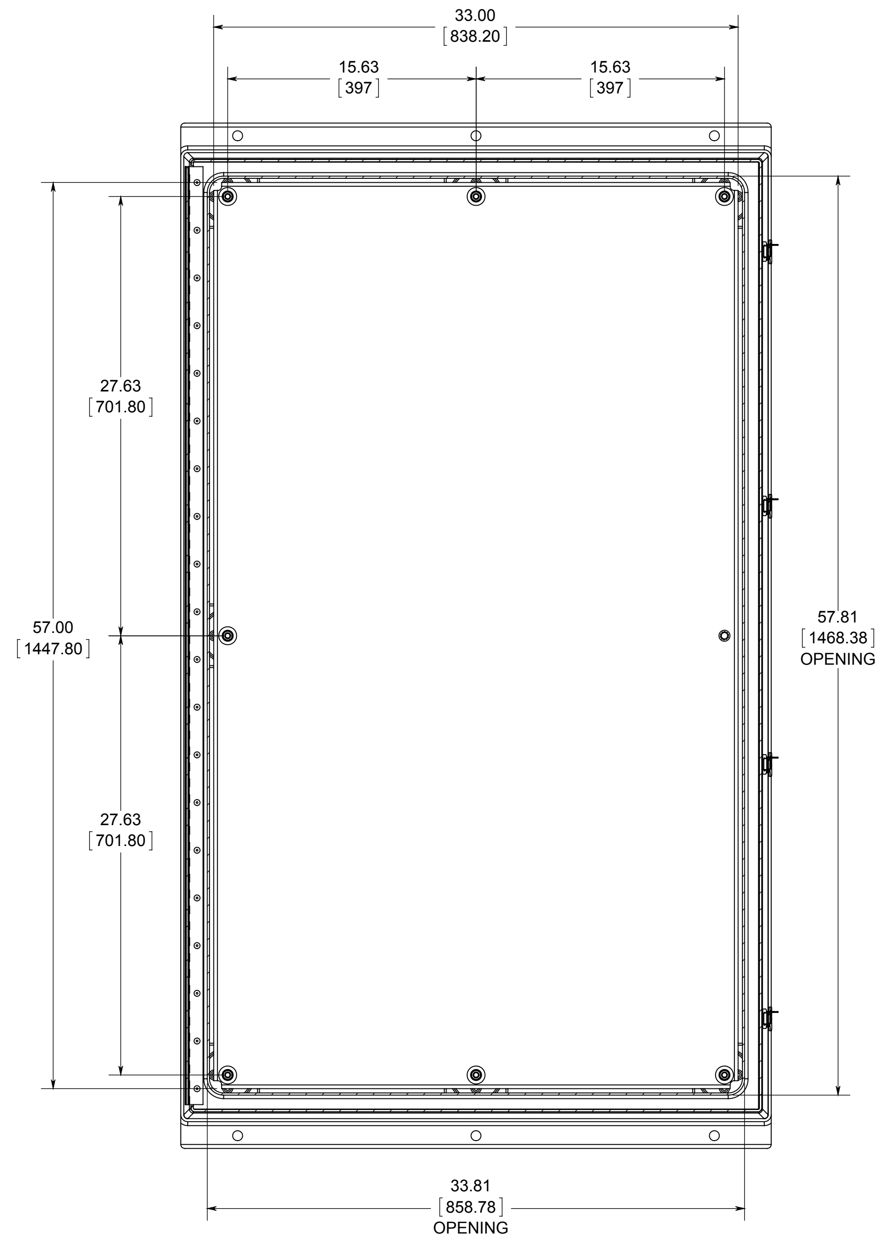
SECTION C-C TOP VIEW WITH LID AND GASKET REMOVED
