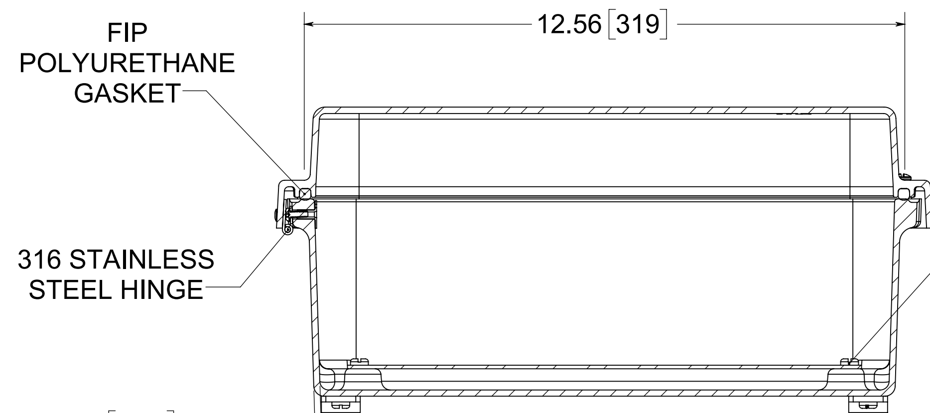
SECTION B-B
