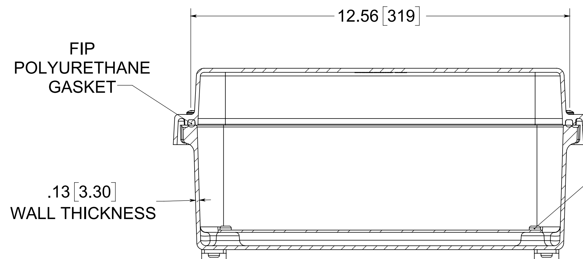
SECTION B-B
