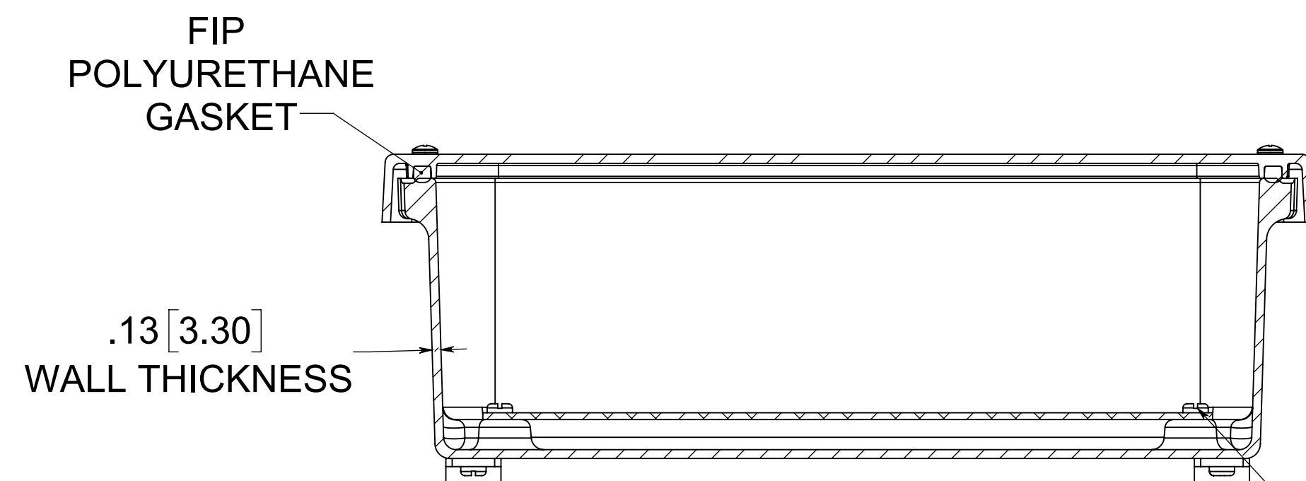
SECTION B-B
