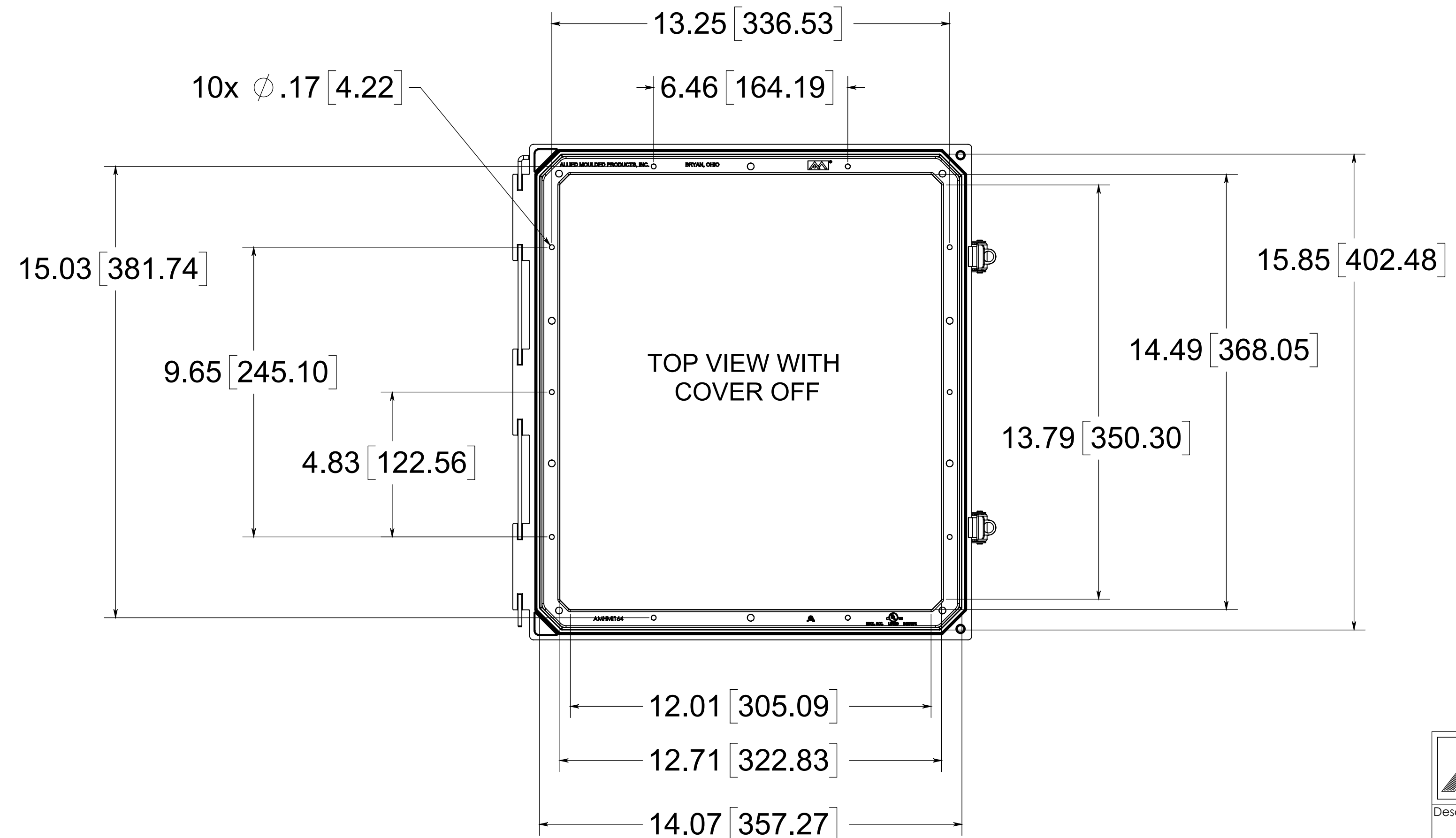
MOUNTING HOLE PATTERN HMI164
