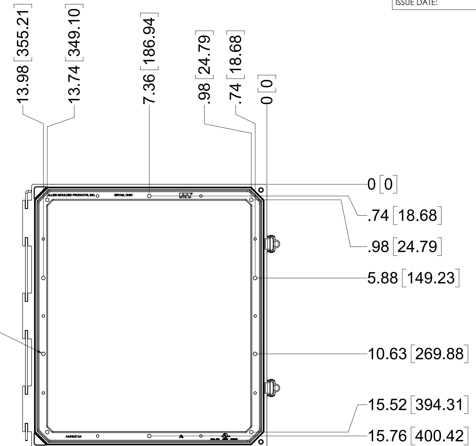
MOUNTING HOLE PATTERN HMI164
