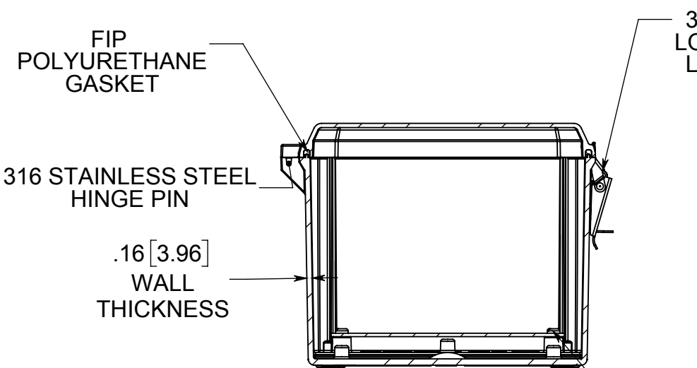
SECTION B-B
