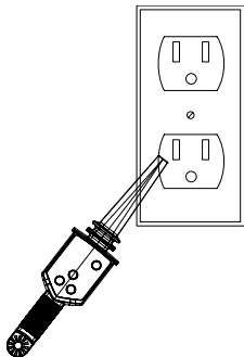
Fig.3 Voltage detection in a outlet (Disconnect all power codes from the outlet)
