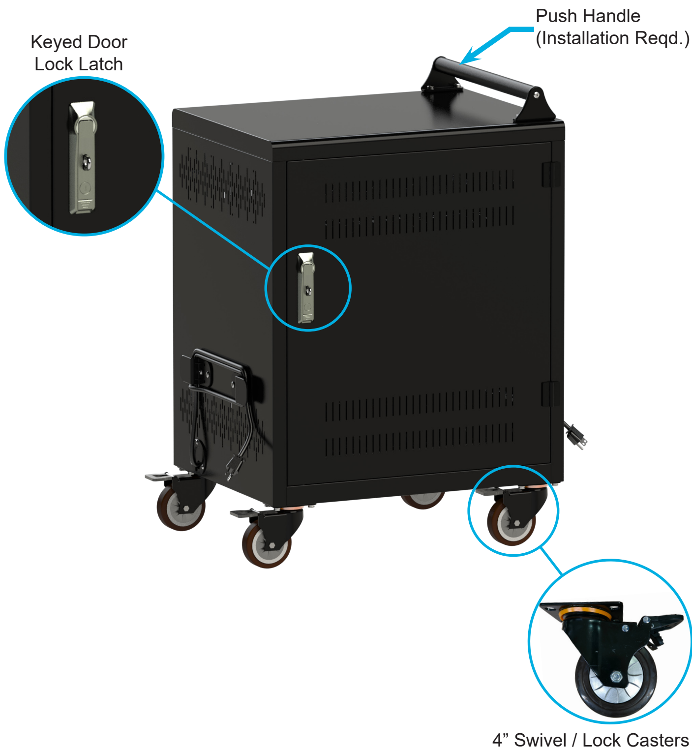
Front View of Cart
