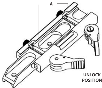
FIGURE 3-6. CO-LR MOUNT. UNDERSIDE VIEW
