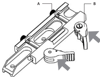
FIGURE 3-7. CLAMPING DEVICE ADJUSTMENT
