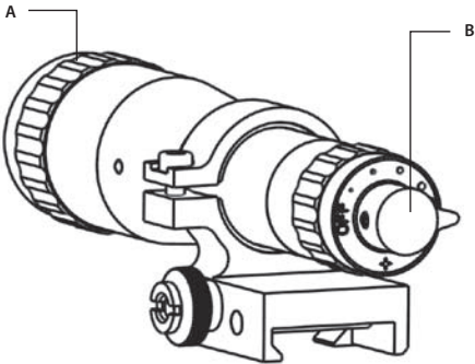
FIGURE 3-14. IR850 CONTROLS
