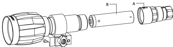
FIGURE 3-10. XLR-IR850 ILLUMINATOR. BATTERY INSTALLATION
