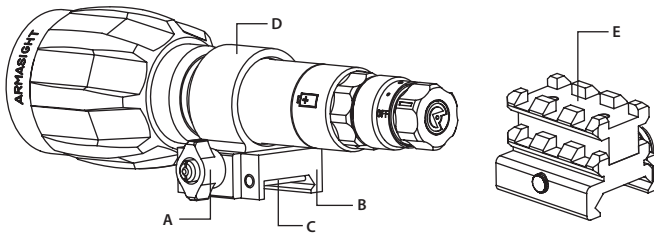
FIGURE 3-8. IR ILLUMINATOR
