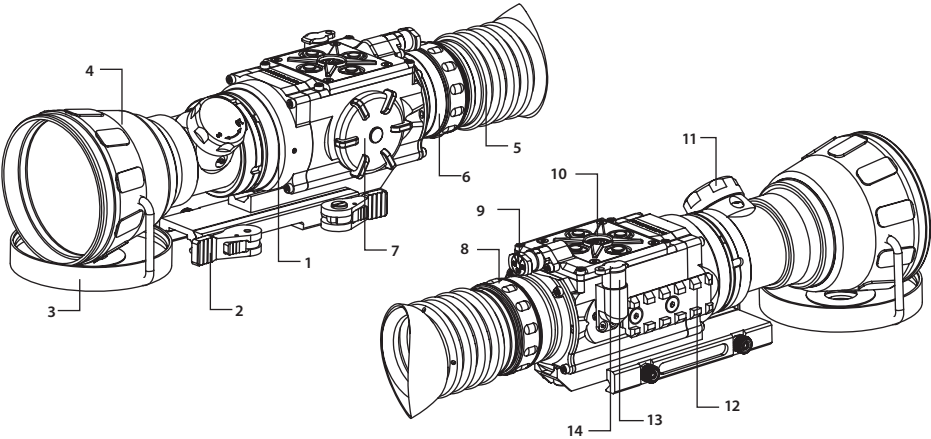
FIGURE 2-2. DRONE PRO DIGITAL NIGHT VISION RIFLESCOPE. SYSTEM DESCRIPTION
