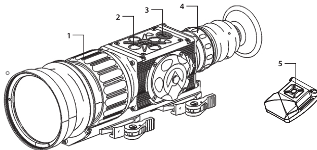
FIGURE 3-9. CONTROLS
