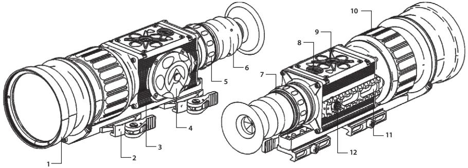
FIGURE 2-2. SYSTEM DESCRIPTION
