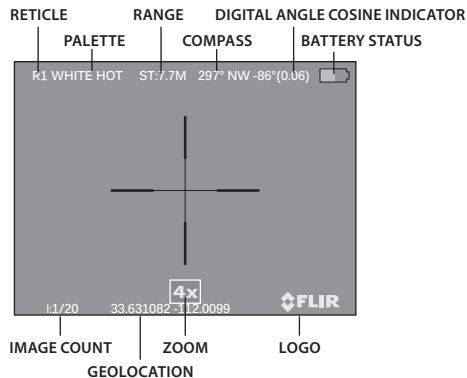
FIGURE 3-24. STATUS VIEW
