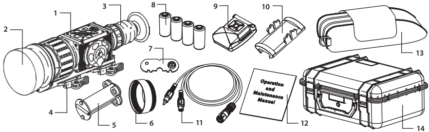
FIGURE 2-3. STANDARD COMPONENTS
