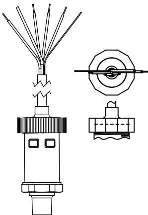
Shielded Cable PVC Jacket, 3' Length Standard, 24AWG Leads
