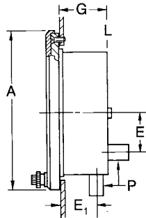
PANEL MOUNTING
