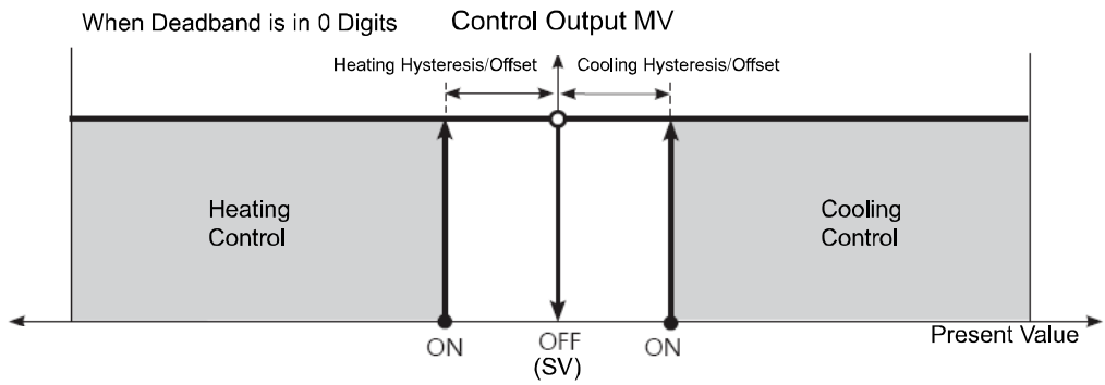
<ON/OFF-ON/OFF Control with Heating and Cooling Control>
