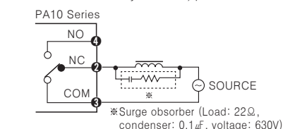
(Picture 1) Relay output
