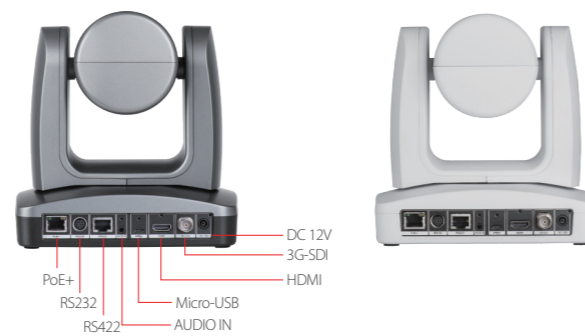
Back Panel
