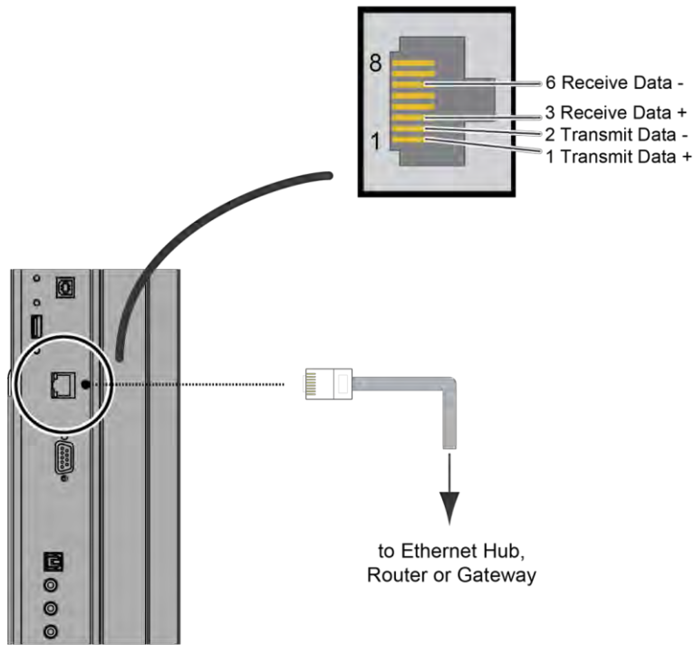
Figure 3-3. Ethernet Connection
