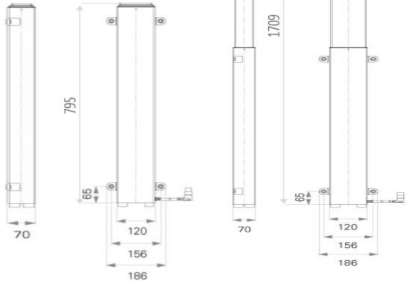
Standard Dimensions (mm)
