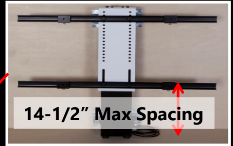
(4) Point Cross Rail Dampening
