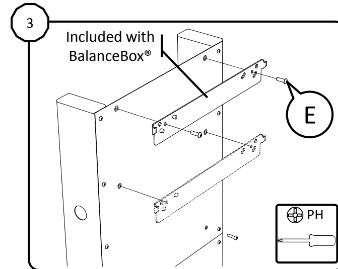
Mount the BalanceBox® bracket ( 2 options for mounting height )
