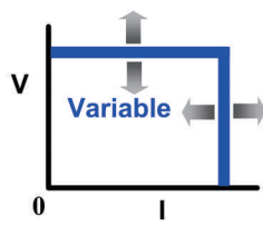
CC+CV Mode
