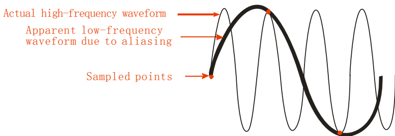
Figure 3.34 – Time Domain Aliasing Illustration
