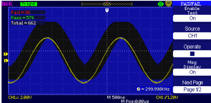
Figure 3.65 – Pass/Fail Screen 2
