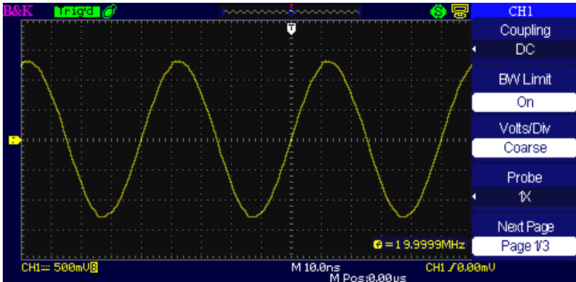
Figure 3.9 – Bandwidth Limit
