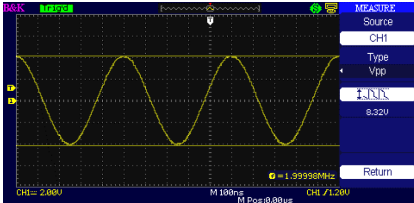
Figure 3.40 – Auto Mode
