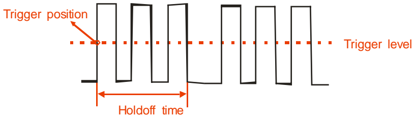
Figure 3.30 – Trigger Holdoff Illustration
