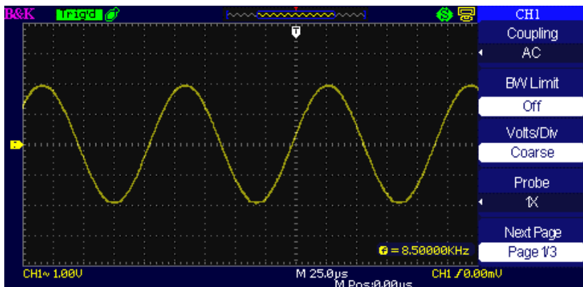
Figure 3.6 – AC Coupling
