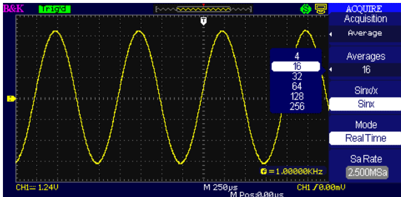
Figure 3.33 – Average Acquisition
