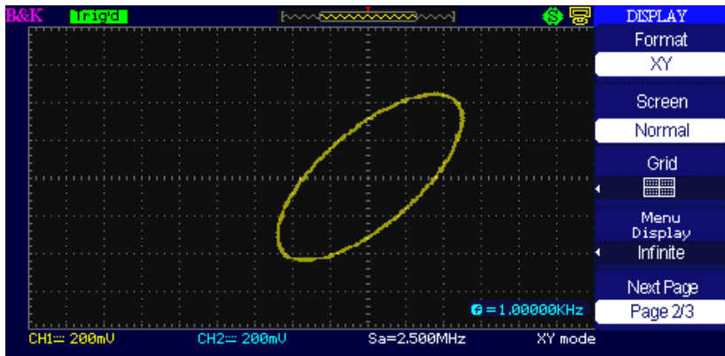
Figure 4.4 – Out of Phase Signals in XY Mode (45 degrees)
