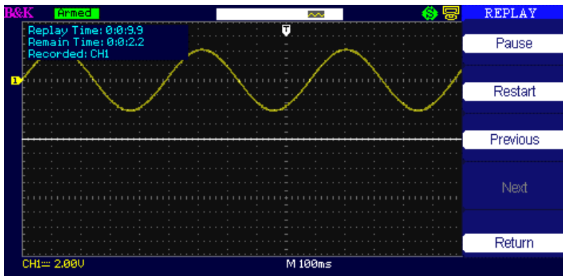
Figure 3.72 – Replay Screen
