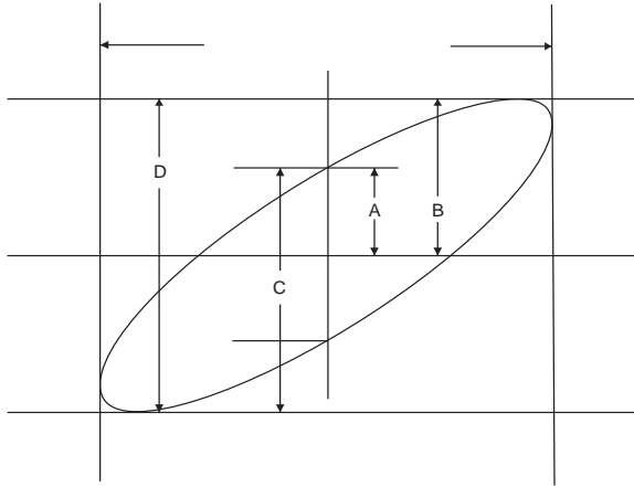
Figure 4.3 - Out of Phase Signals (45 degrees)
