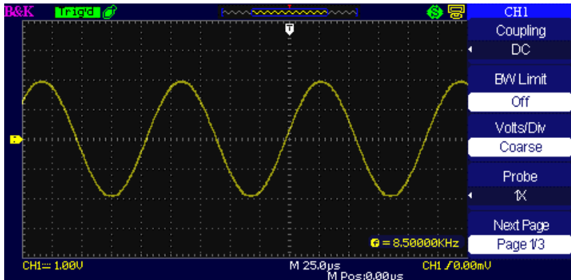
Figure 3.7 – DC Coupling
