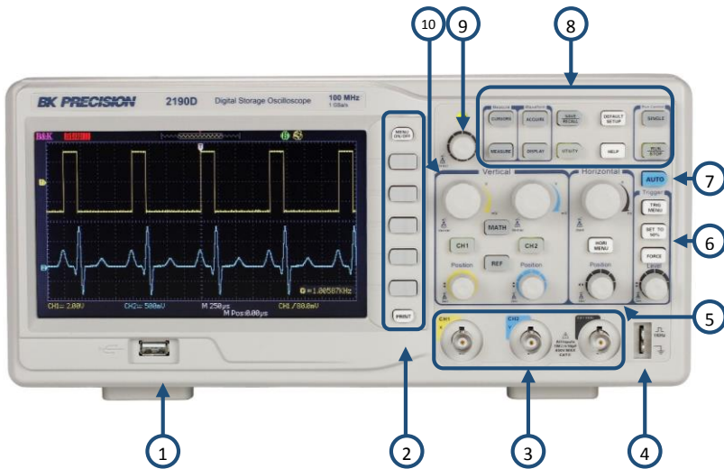
Figure 1.1 – Front Panel
