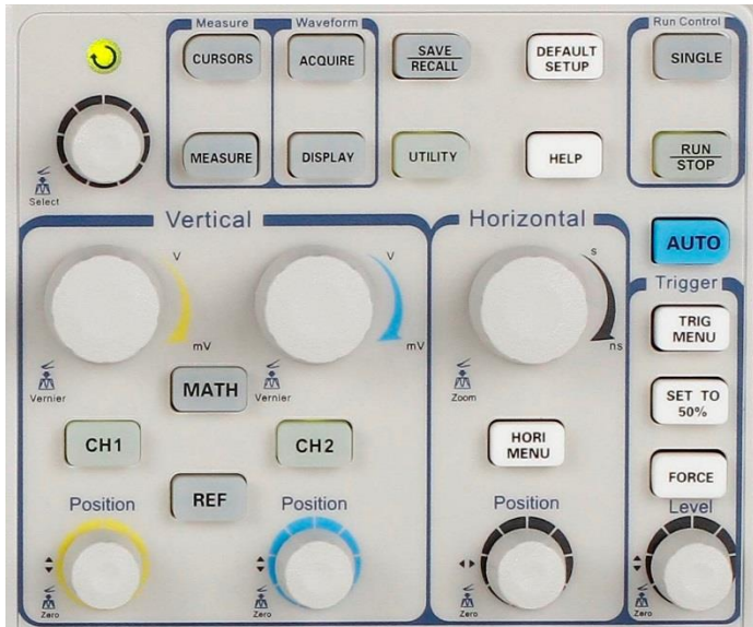
Figure 3.1 – Control Buttons
