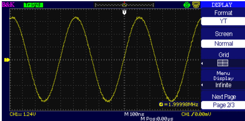
Figure 3.36 – Display Menu 2
