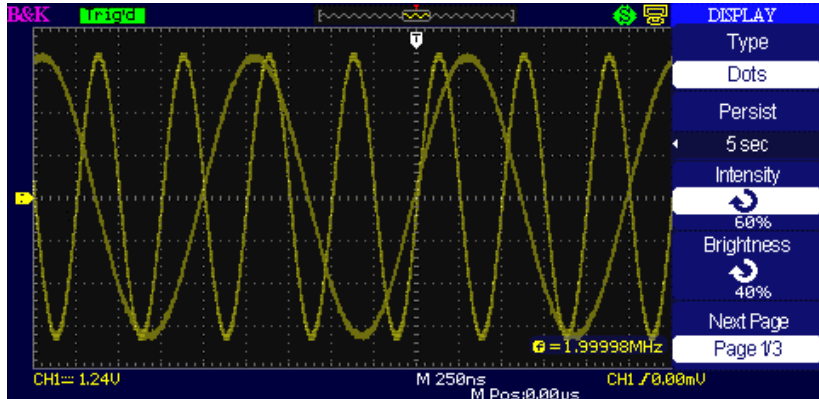
Figure 3.37 – Persist Screen
