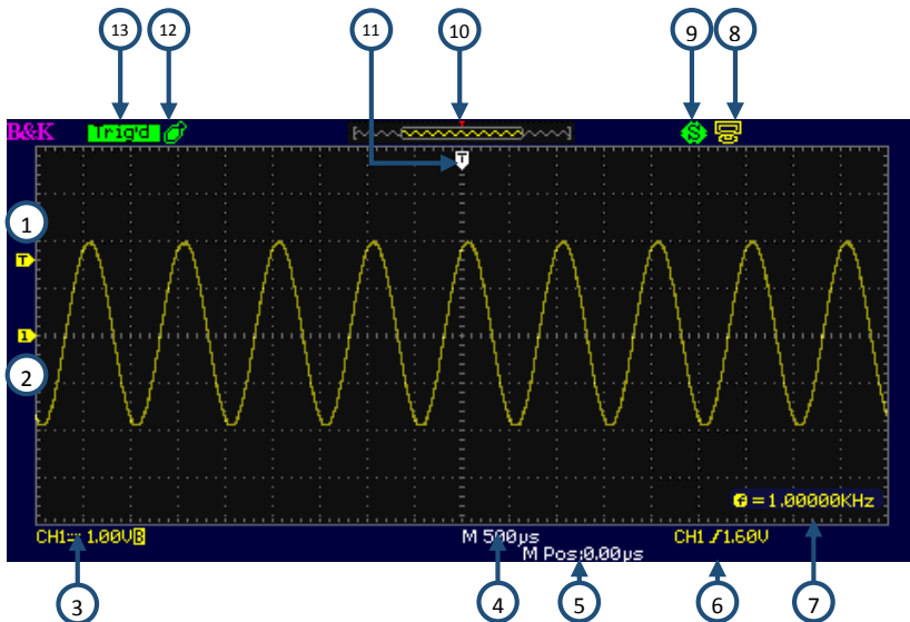
Figure 1.3 – Display Screen
