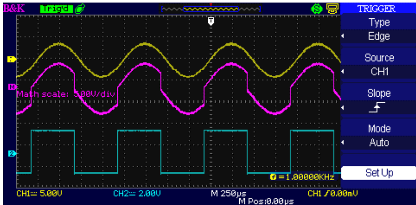
Figure 3.15 – Math Waveform
