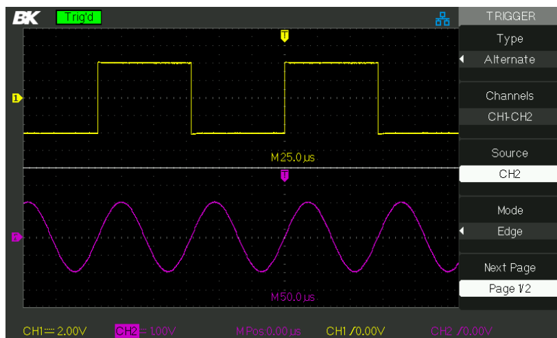
Figure 3.27 – Alternate Trigger Menu
