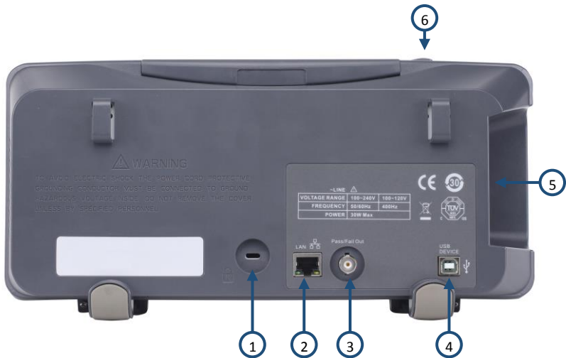
Figure 1.2 – Back Panel
