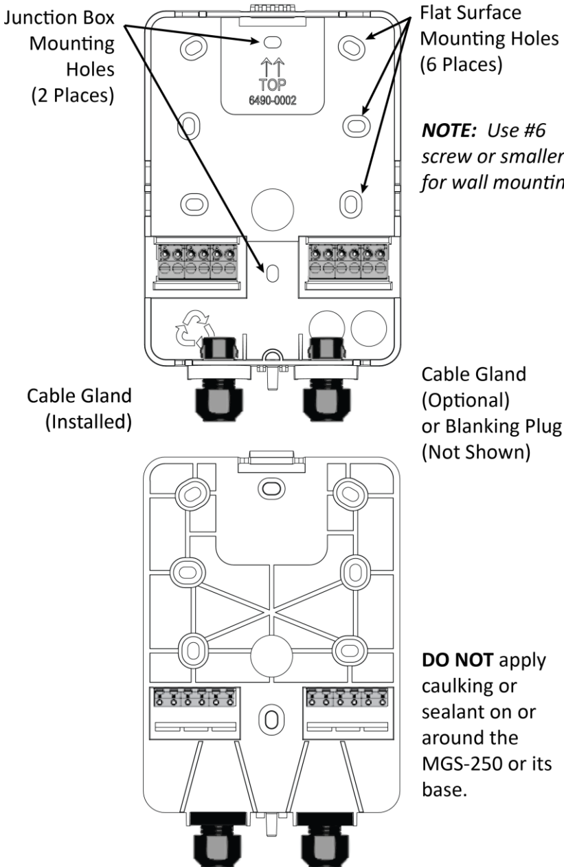
Figure 4. Front and Back Views of MGS-250 Base
