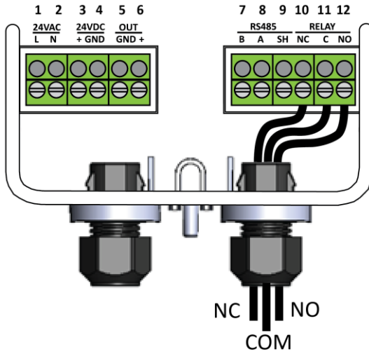
Figure 9. Sample Relay Output Wiring
