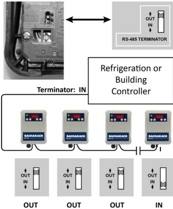
Figure 11. Setting Network Termination Resistors
