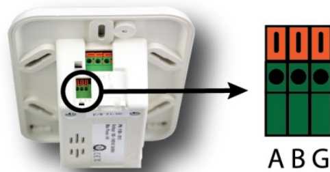
Figure 8. Modbus Wiring Terminals
