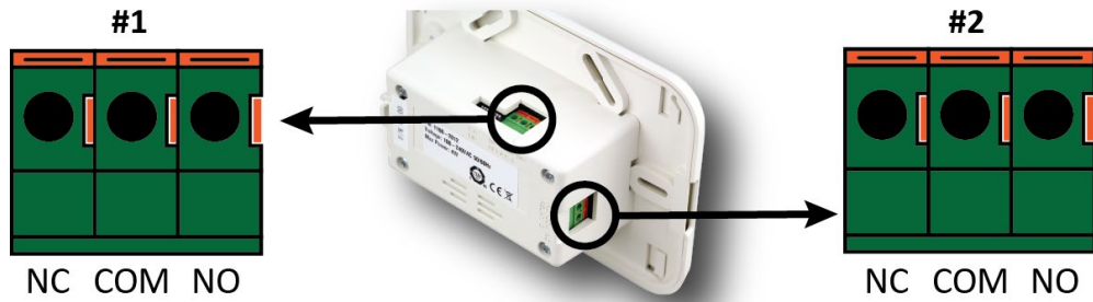
Figure 7. Wiring Relay 1 (Low Gas Alarm) and Relay 2 (High Gas Alarm or Fault)
