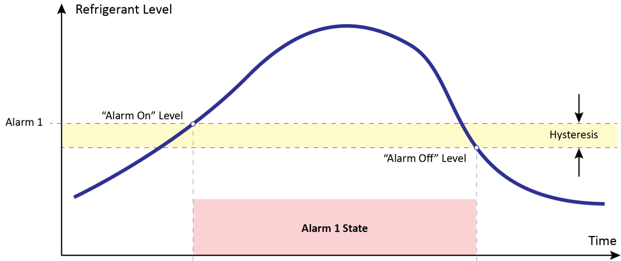
Figure 13. Default Alarm Generation
