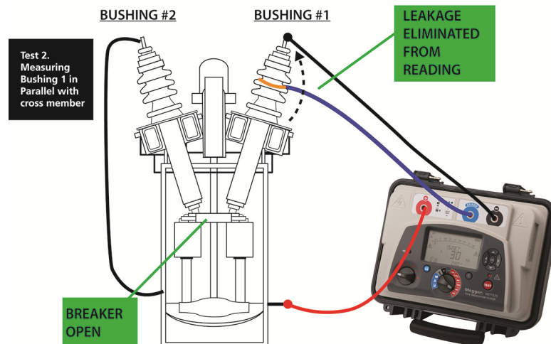
Figure 11: Measuring bushing 1
